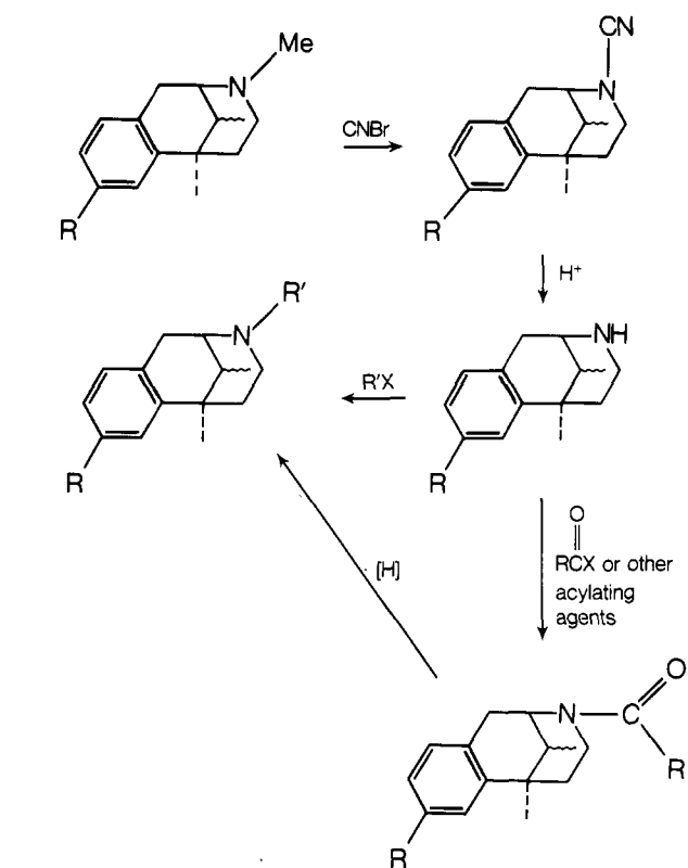
SCHEME VIII. Routes to N-Substituted Benzomorphans
